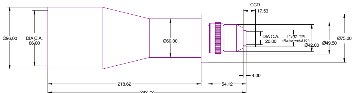
Figure 2: outline drawing
