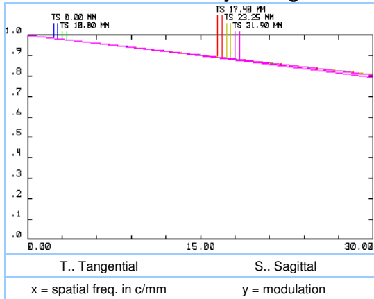
MTF for various object heights
