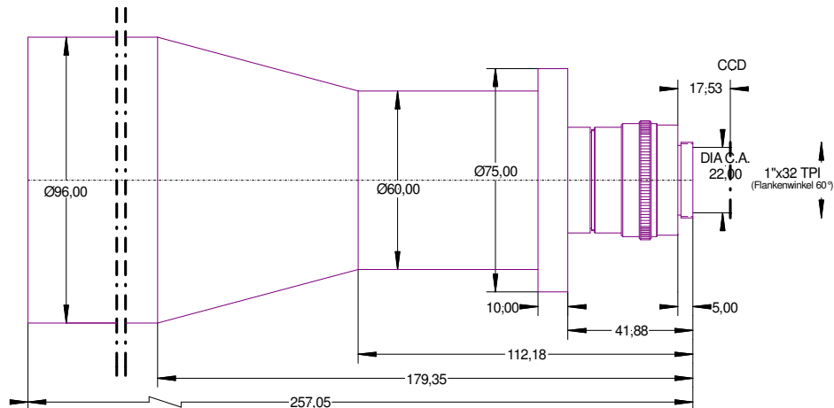
Figure 2: outline drawing
