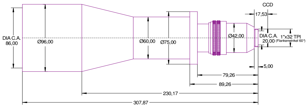
Figure 2: outline drawing
