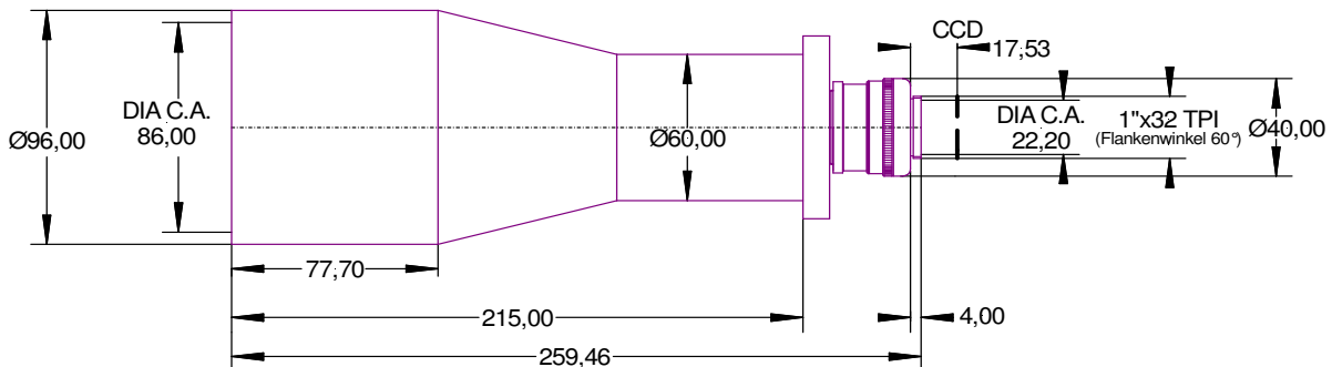
Figure 2: outline drawing
