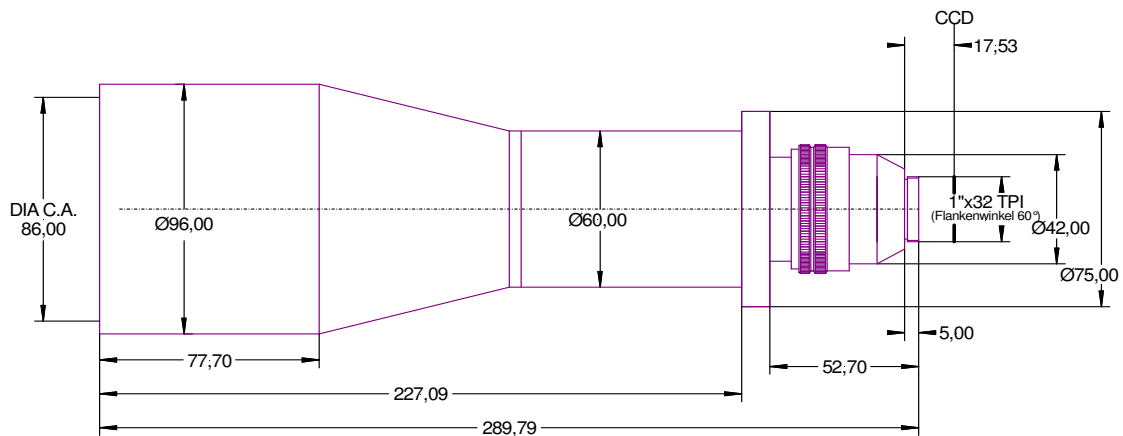
Figure 2: outline drawing
