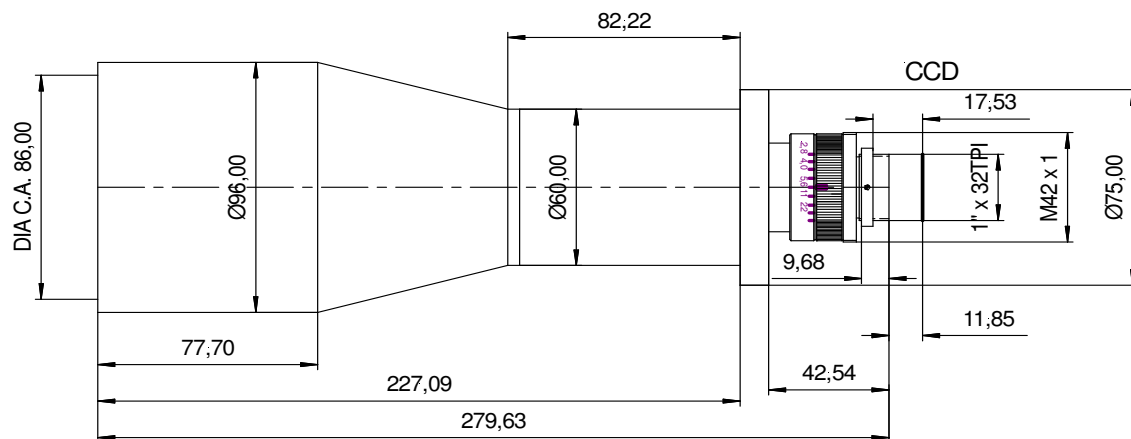
Figure 2: outline drawing
