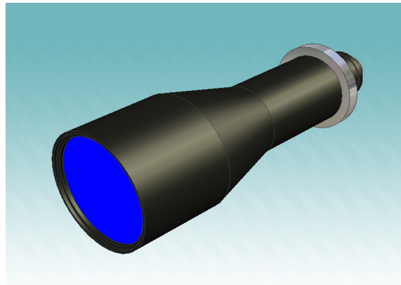
Figure 1: telecentric lens
