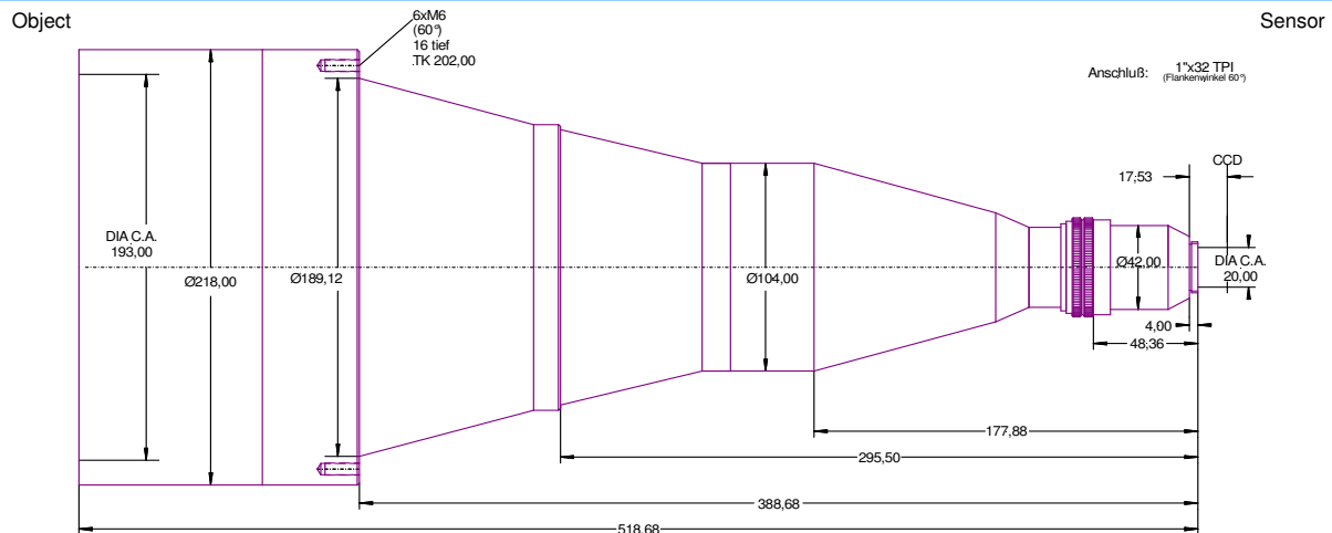
Figure 2: outline drawing
