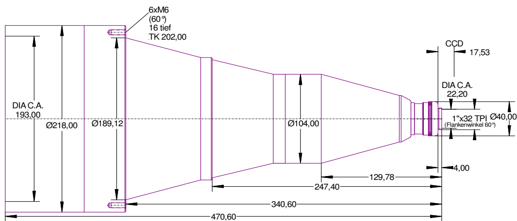
Figure 2: outline drawing
