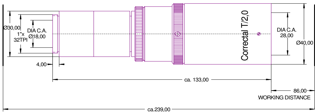
Figure 2: outline drawing
