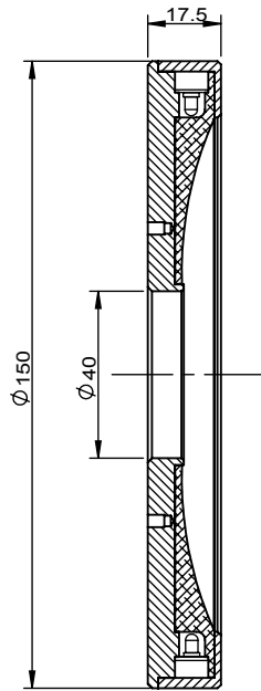
Sectional View A-A
