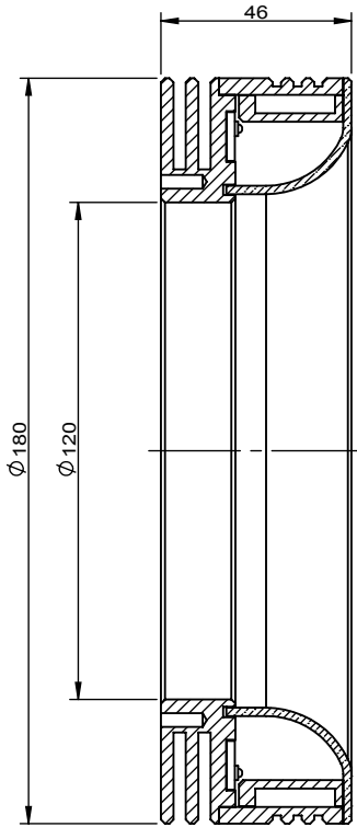
Sectional View A-A
