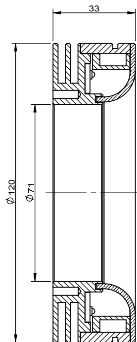
Sectional View A-A
