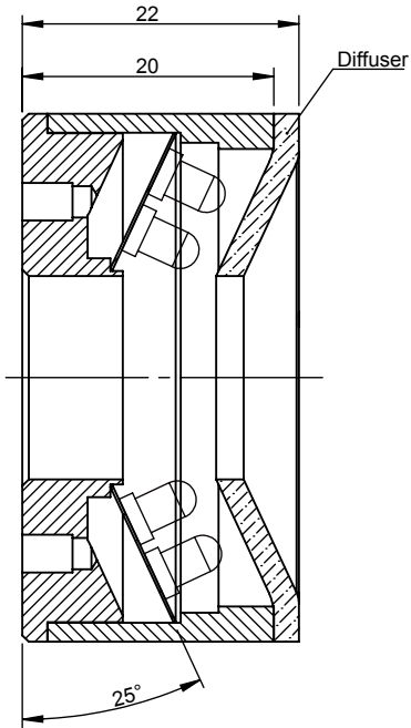
Sectional View A-A
