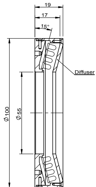
Sectional View A-A
