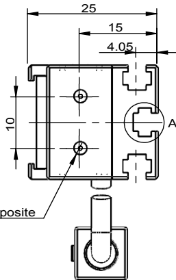
Partial View A scale 3 : 1
