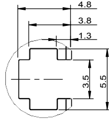
Partial View A scale 3 : 1
