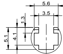
Partial View A scale 2 : 1
