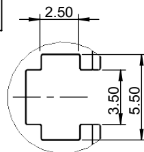
Partial View A scale 3 : 1
