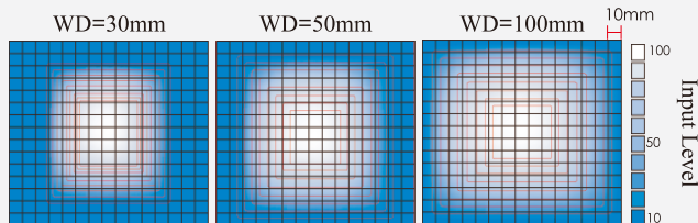
OPT-CO50-RGB Uniformity Chart
