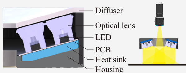
RGB Ring Light Section Structure and Illumination
