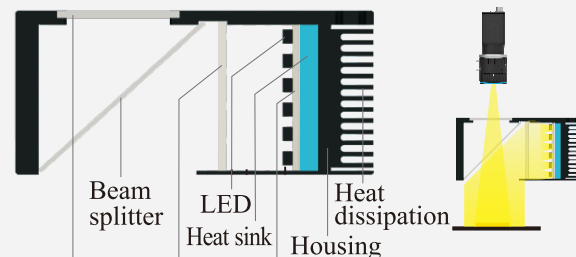
RGB Coaxial Light Section Structure and Illumination
