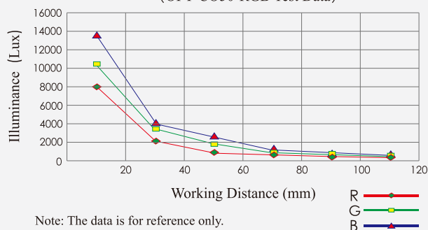
Intensity Comparison at Different Working Distances (OPT-CO50-RGB Test Data)
