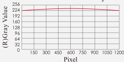
OPT-FL9090-G Uniformity Chart
