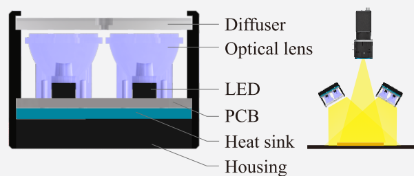
RGB Bar Light Section Structure and Illumination
