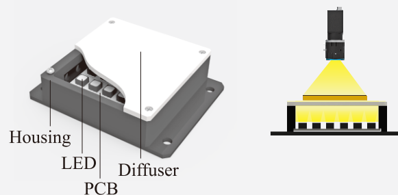
RGB Bottom Backlight Section Structure and Illumination
