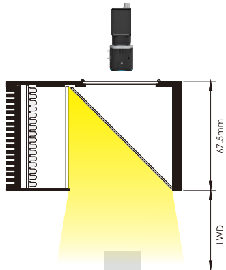
Coaxial light OPT-CO70
