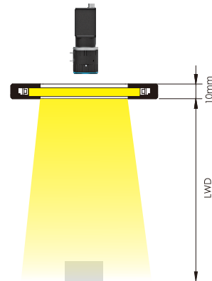
Flat dome light OPT-FC100
