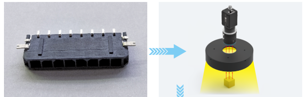
Workpiece
