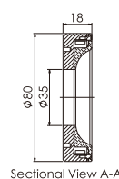
Sectional View A-A
