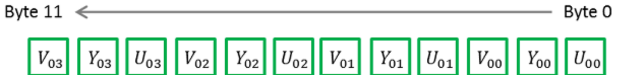
Figure 5. Packing format for YUV444Packed.
