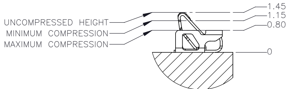
DETAIL C COMPRESSION SPRING SCALE 12:1
