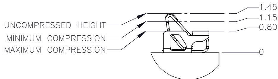
DETAIL C COMPRESSION SPRING SCALE 12 : 1
