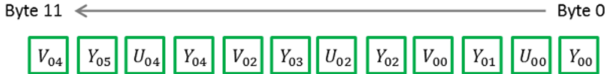
Figure 7. Packing format for YCbCr422_8 .
