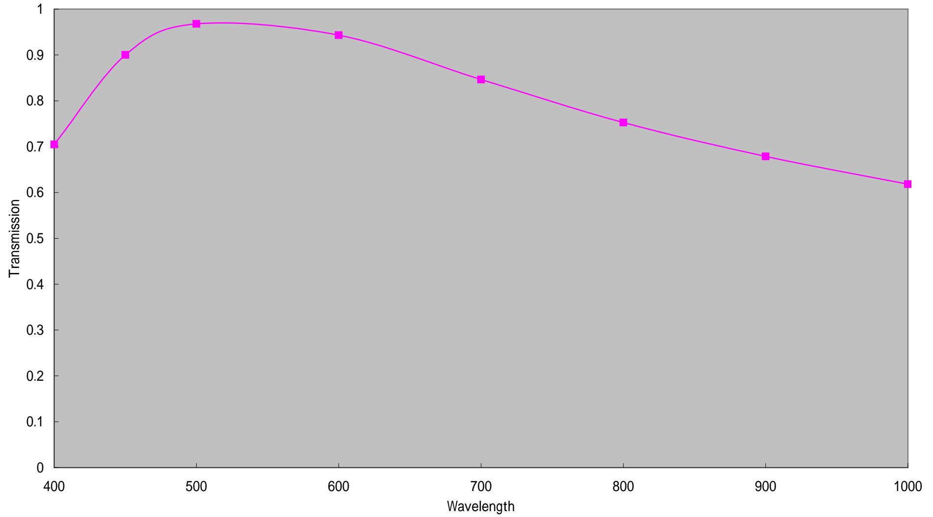
LM16JC (970) Transmission
