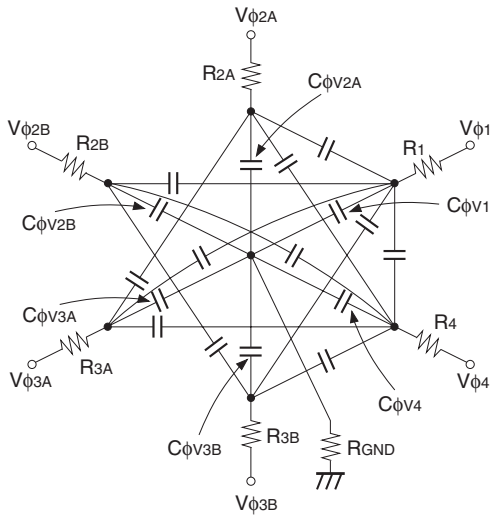
Vertical transfer clock equivalent circuit
